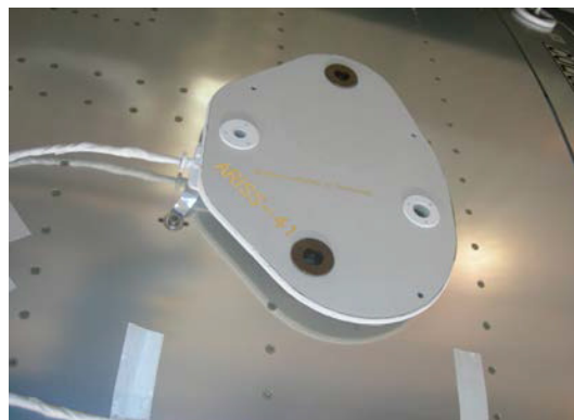
ARISS L/S-band patch antenna
